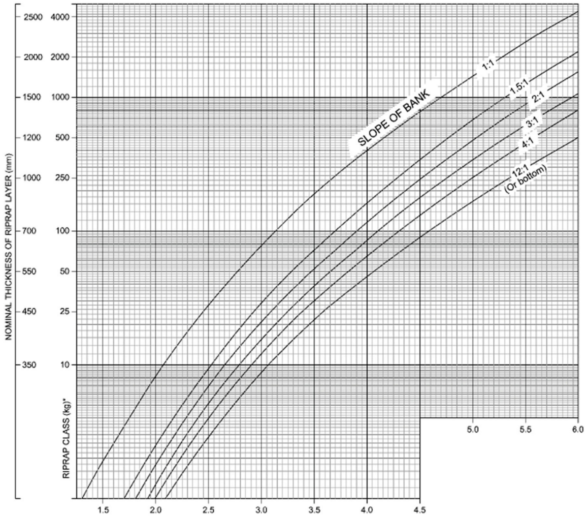
FIGURE M-2 RIPRAP DESIGN CHART
